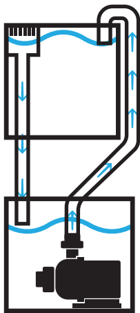
Return Pump
