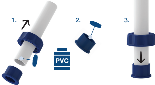
Union Coupling
